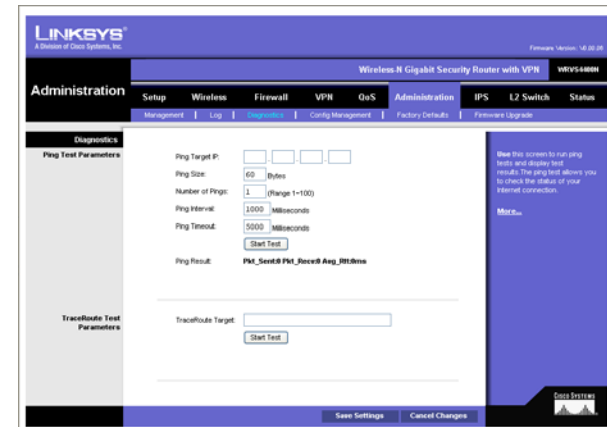
Figure 6-52: Administration - Diagnostics
